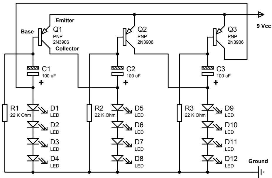
TREE Astable Multivibrator
